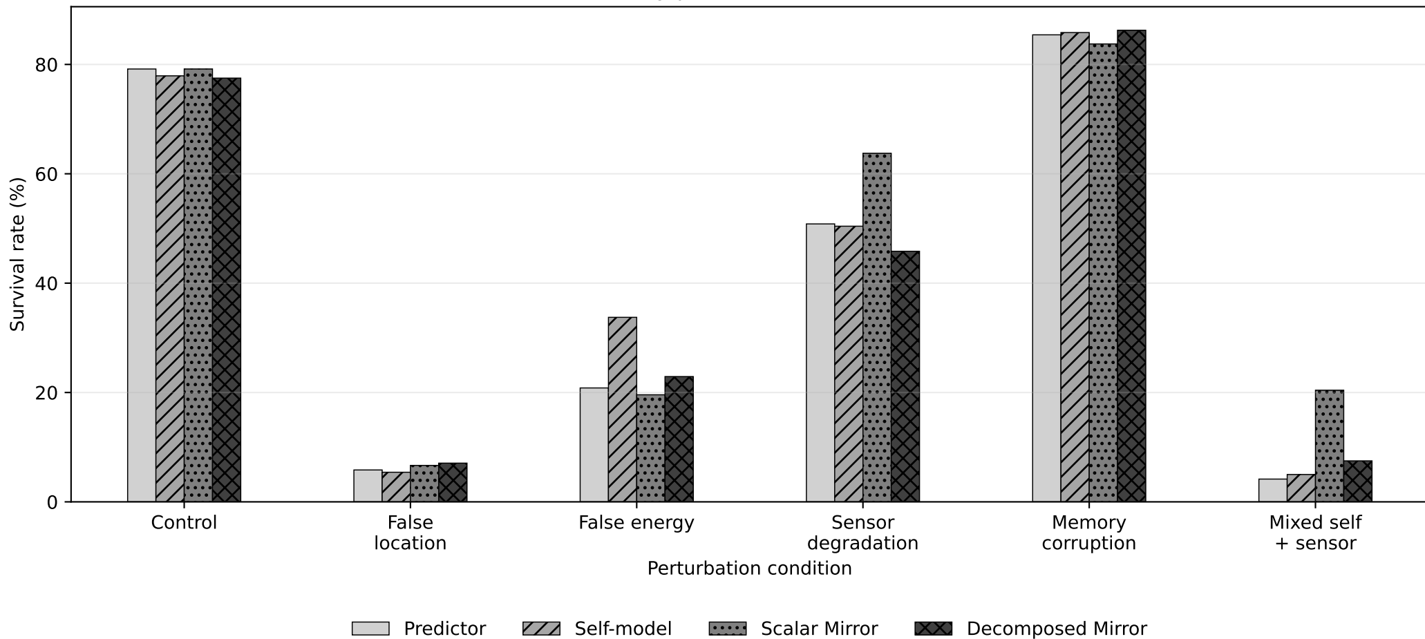
Survival rate by perturbation and architecture
